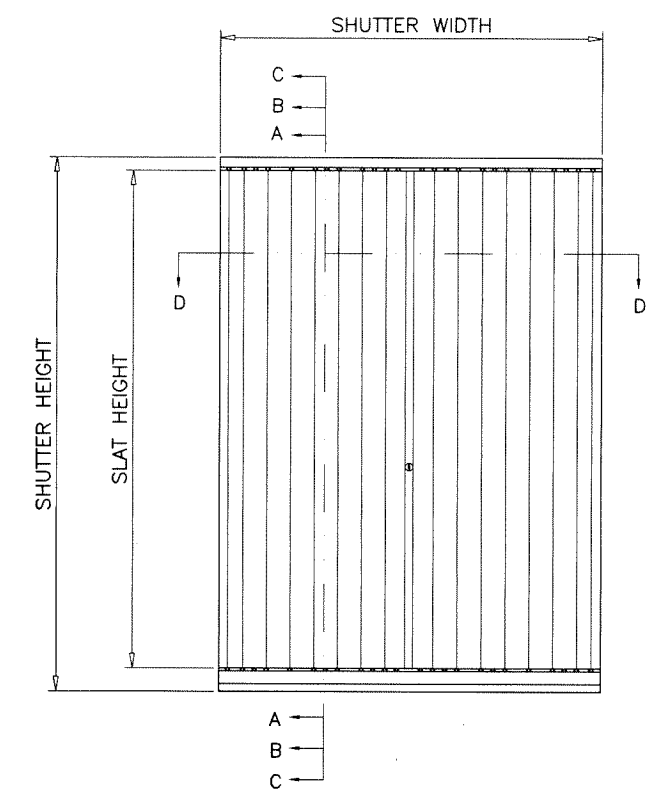
TYPICAL ELEVATION
