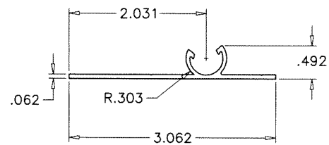
FEMALE END SLAT 6063-T6
