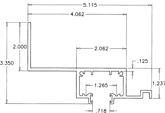
2" BUILT-OUT WALL HEADER 6063-T6
